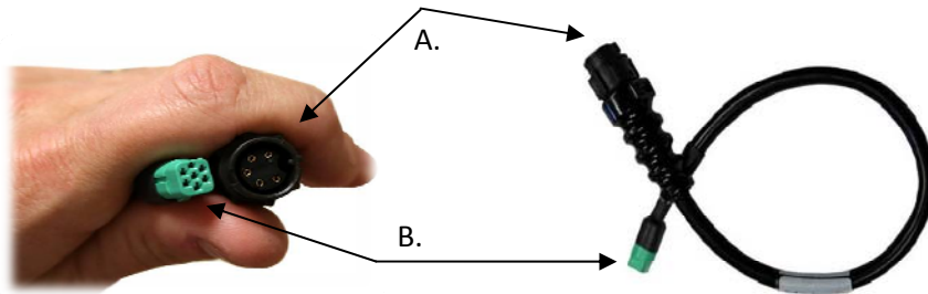
A. 7-pin Female Green Mini Amp Machine Connector B. 5-pin Female Switchcraft Connector
